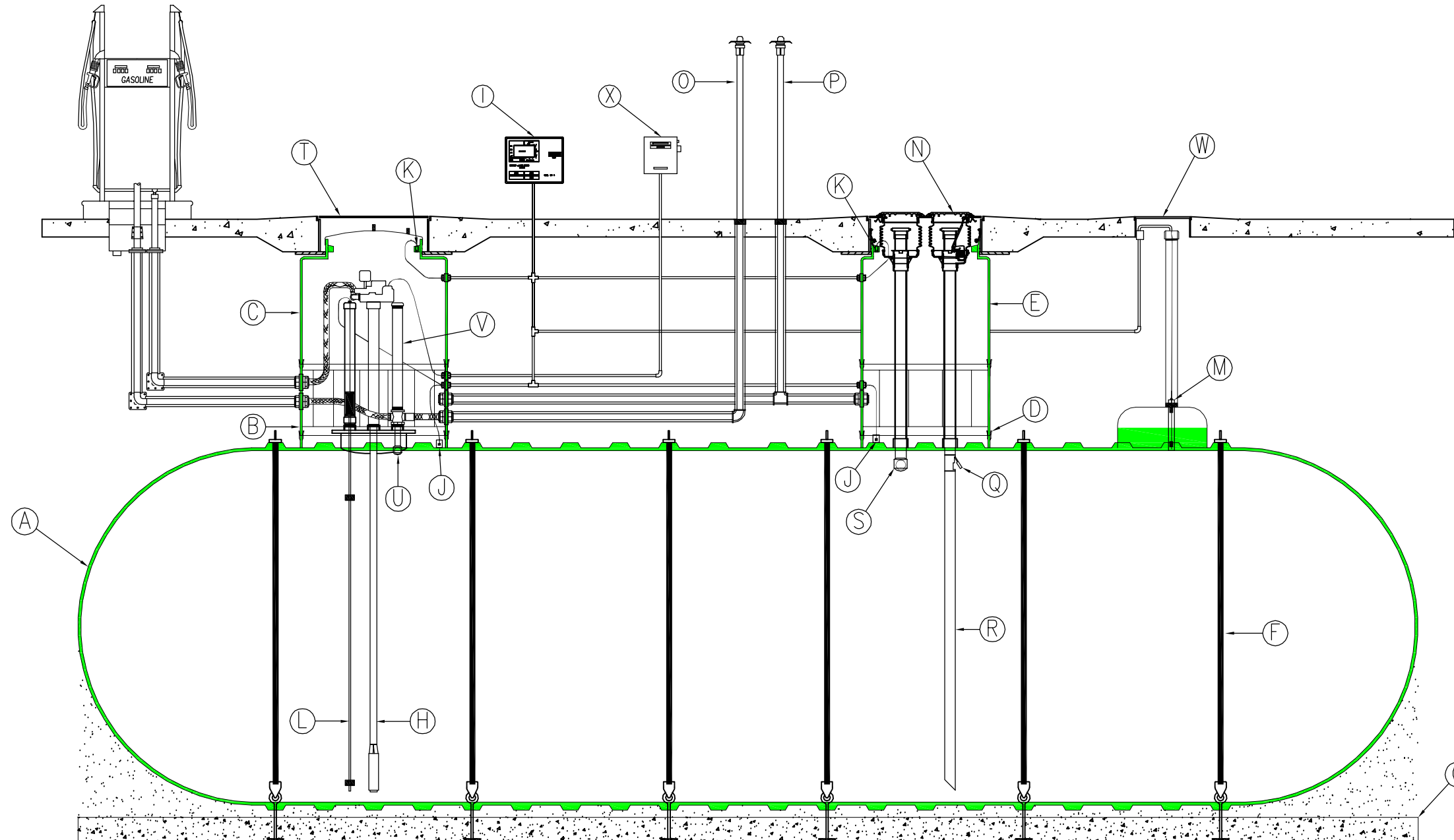
TYPICAL ILLUSTRATION DRAWING DWT-6 TYPE II (10') 20,000
